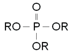
-triester
