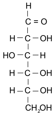
D-Glucose
