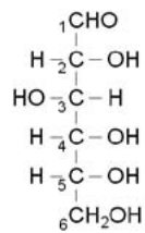
D-Glucose
