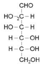
D-Mannose
