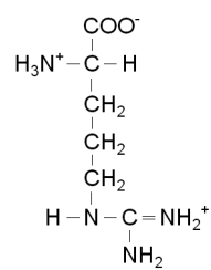
Arginin
