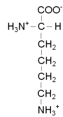
Lysin
