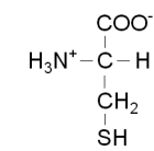
Cystein
