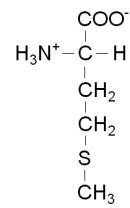
Methionin
