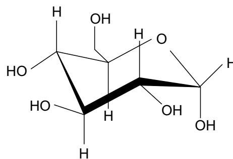
\alpha -D-Glucose
