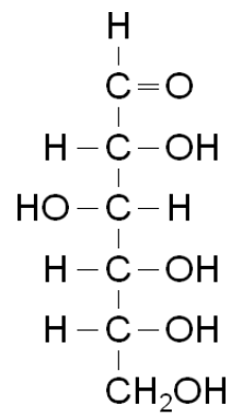
D-Glucose
