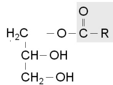
Monoacylglycerid
