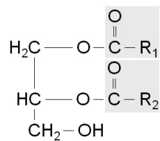
Diacylglycerid
