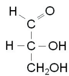
D - Glycerinaldehyd
