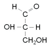
L - Glycerinaldehyd
