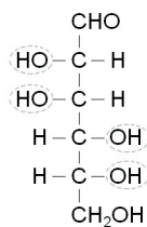
D - Mannose
