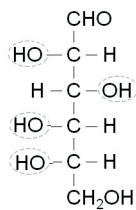
L - Glucose
