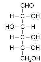
D - Glucose
