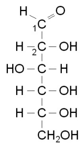
D-Glucose
