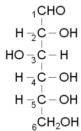
D-Glucose
